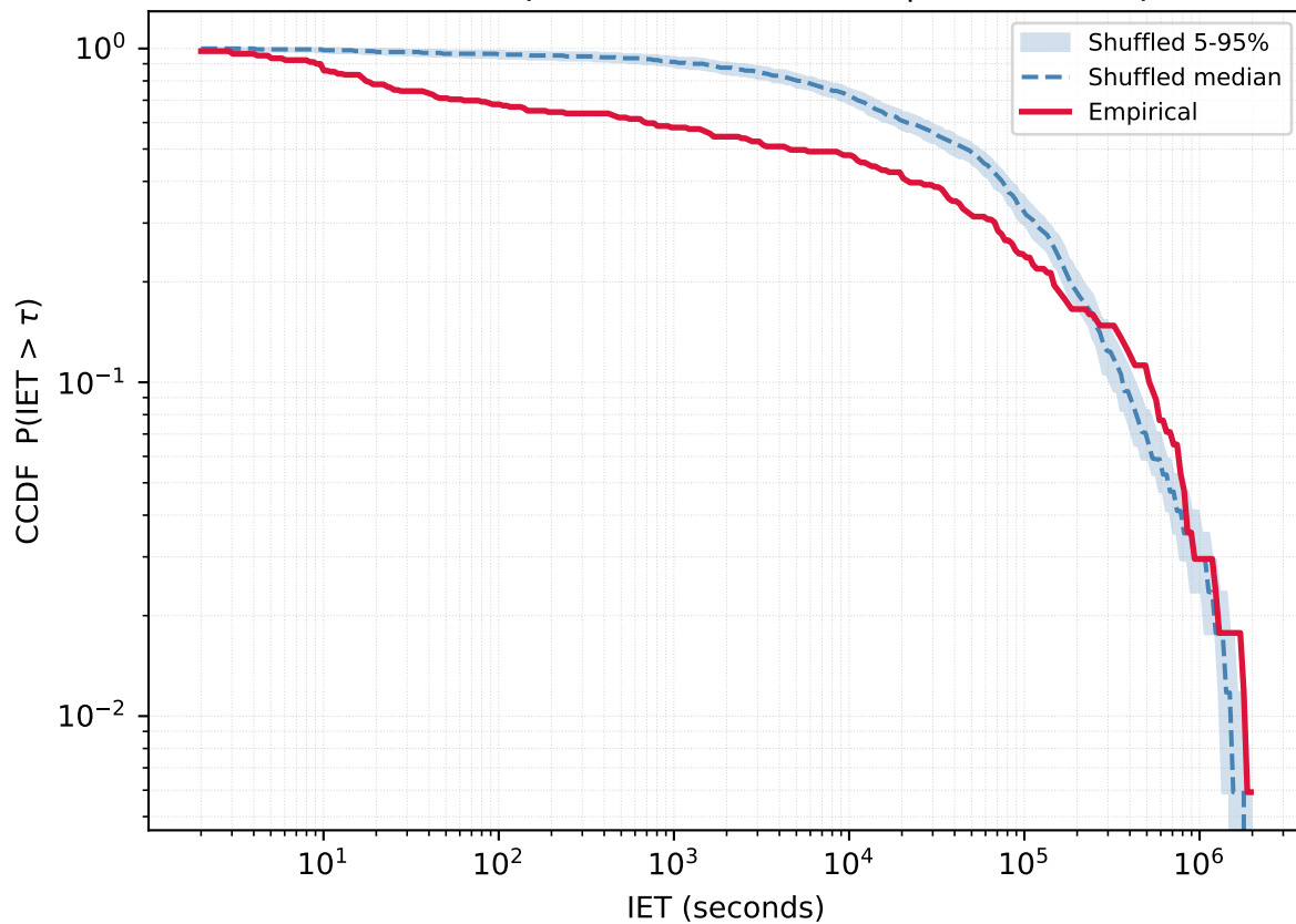
User 32432053 - Empirical vs Reshuffled | KS=0.348 p=0.000
